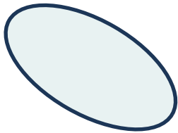
Ellipse: setRotation
